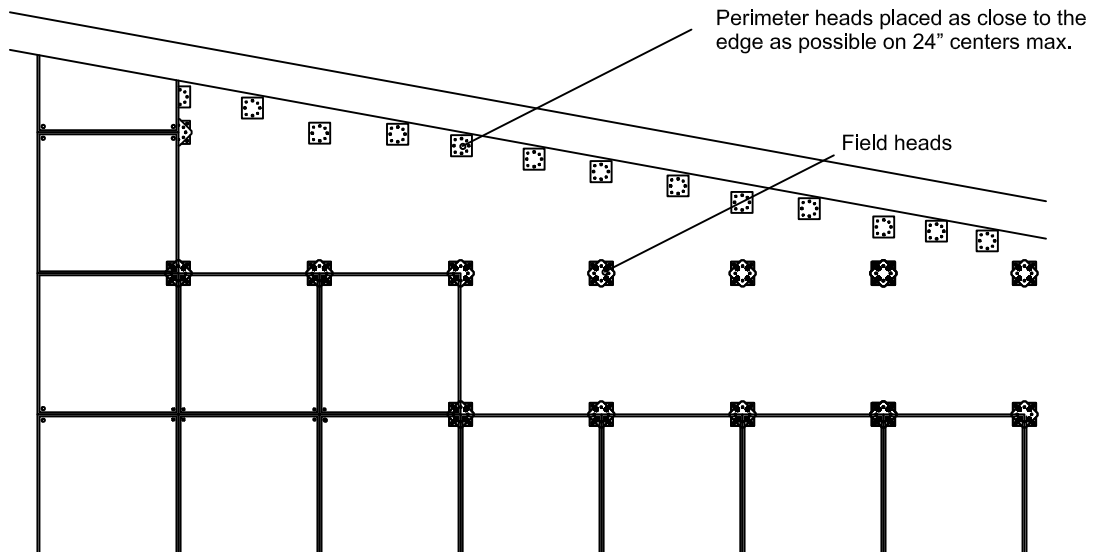
Perimeter Condition at Angled Wall without Stringer
