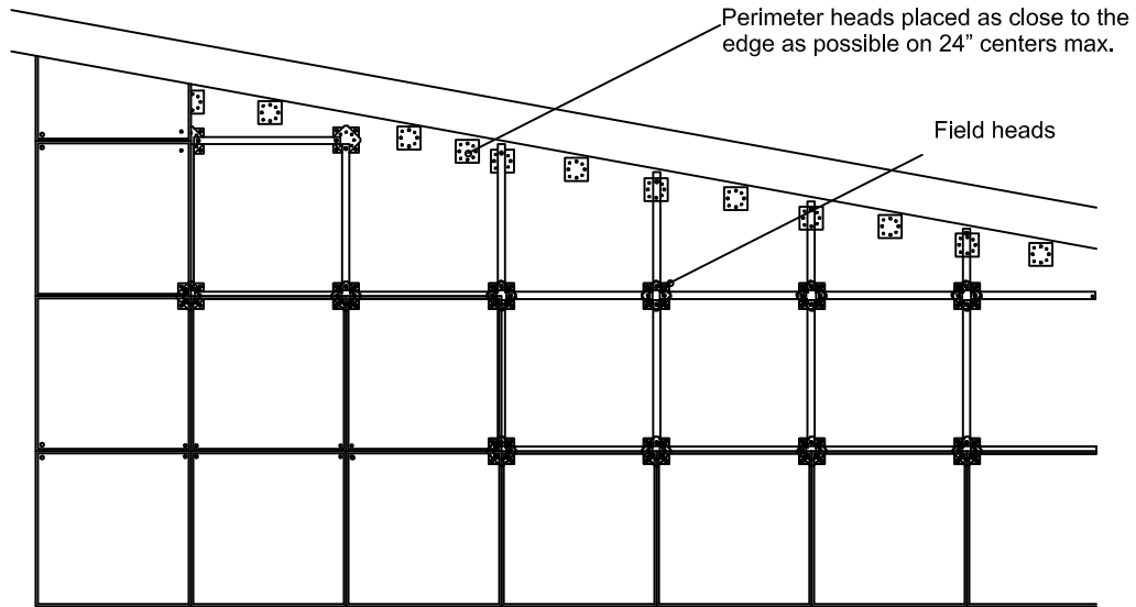
Perimeter Condition at Angled Wall with Stringer
