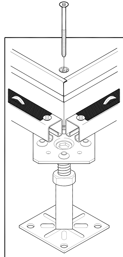
Typical Bare TecCrete Corner Lock Configuration
