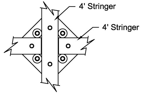
TYPICAL INTERSECTION SCALE: 1 : 4
