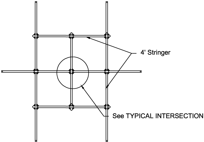
Standard 4' Basketweave Layout
