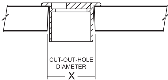
SECTION VIEW
