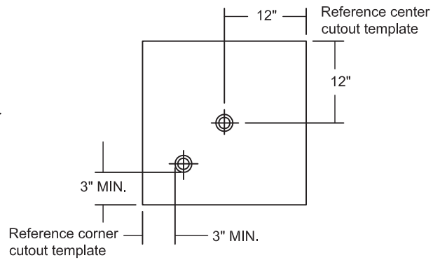
STANDARD CUTOUT LOCATIONS
