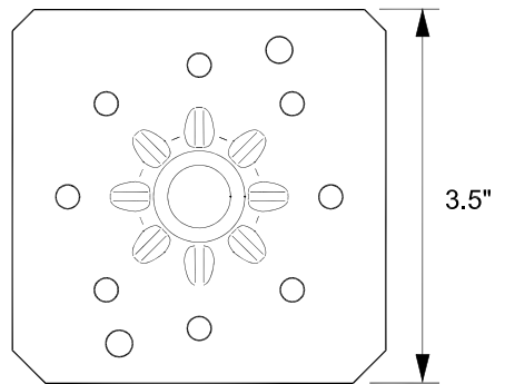
TOP VIEW OF PEDESTAL BASE
