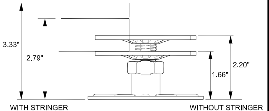
LOW PROFILE HEIGHT
