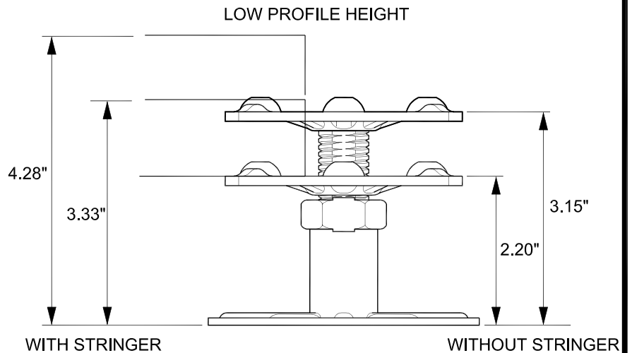
PERIMETER PEDESTAL HEAD LOW PROFILE 4"
