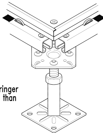
Corner-Lock Application
