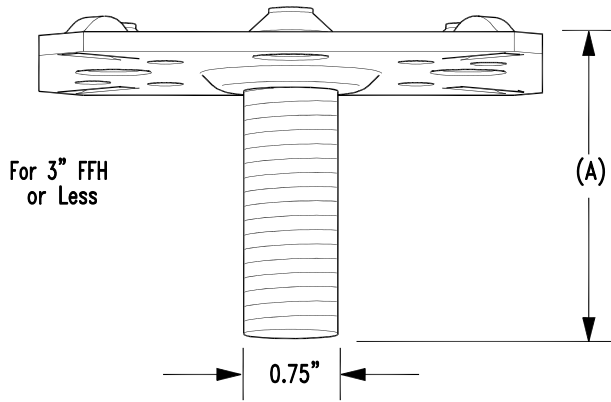
(Low Profile)
